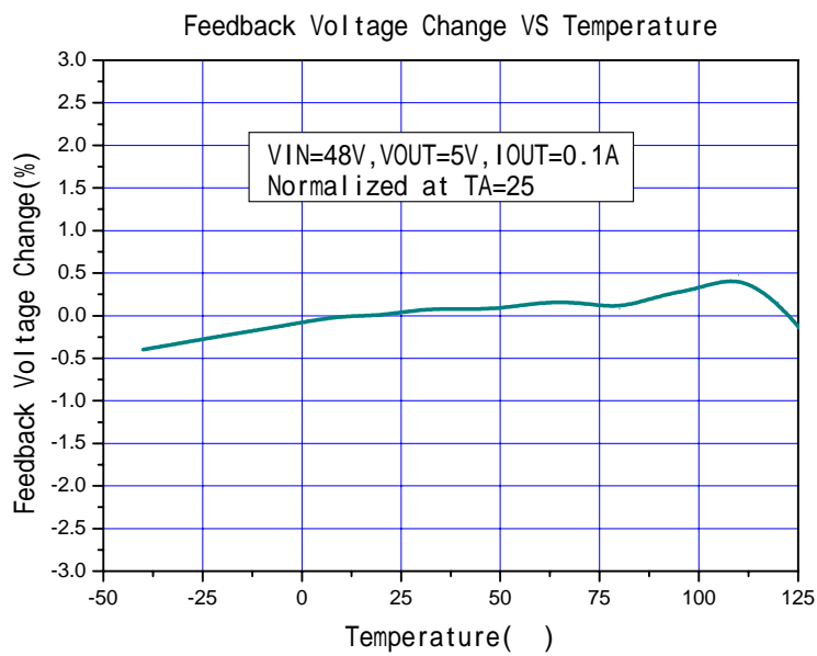
Figure6. Feedback Voltage Curve
