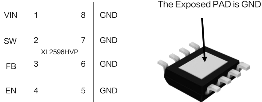
Figure2. Pin Configuration of XL2596HVP
