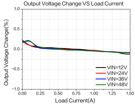
Figure15.Load Regulation
