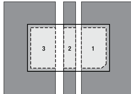
Dark grey areas show added PCB copper area for better thermal resistance.
