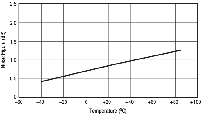
Figure 8. Noise Figure vs Temperature
