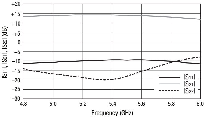
Figure 3. S-Parameter Data
