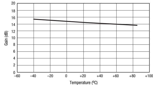
Figure 7. Gain vs Temperature
