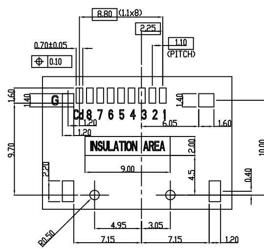
RECOMMEND PCB BOARD LAYOUT
