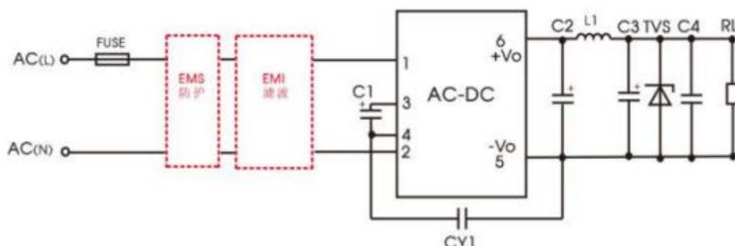
LS05(-F) series peripheral device selection reference (excluding EMC devices)
