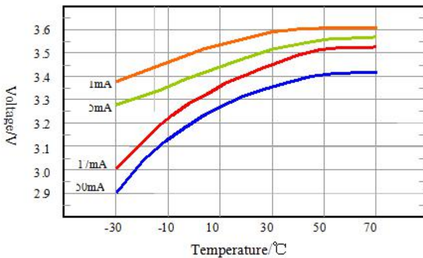
Voltage performance at different temperature
