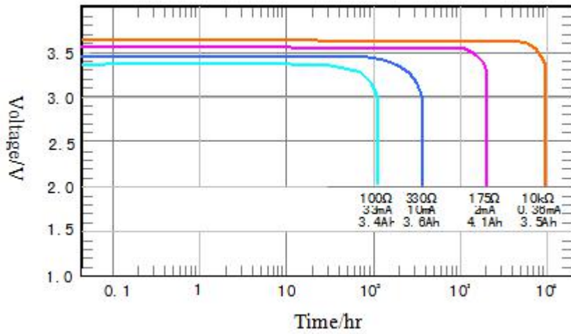
Discharge capacity performance at different discharge current
