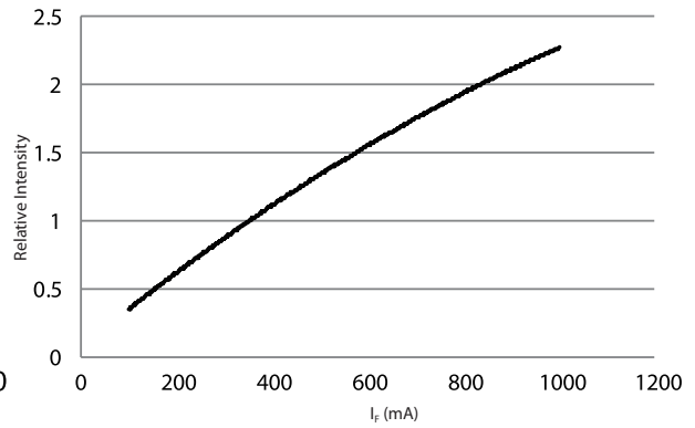
Figure 12. Relative luminous flux vs. forward current for Cool White
