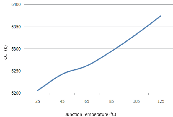
Figure 8. Typical CCT vs. junction temperature for Cool White.
