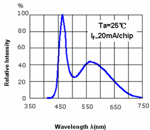
< Figure 4 Wavelength & relative intensity for PLCC 3528 series.>
