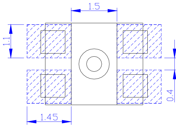
<Figure 9 Pad Dimension >
