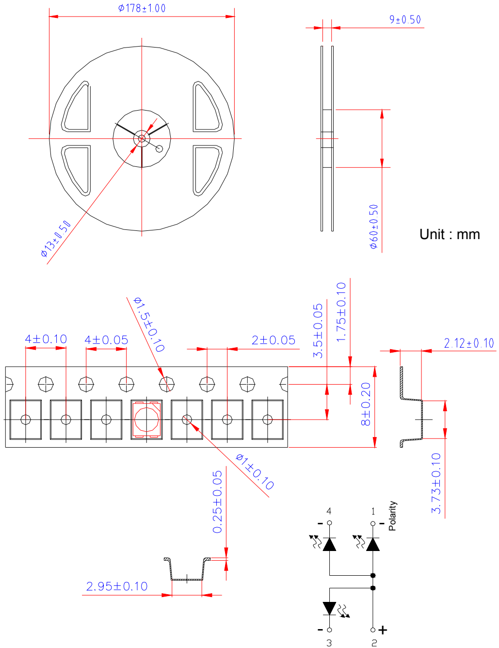
< Figure 11 Taping reel dimensions >
