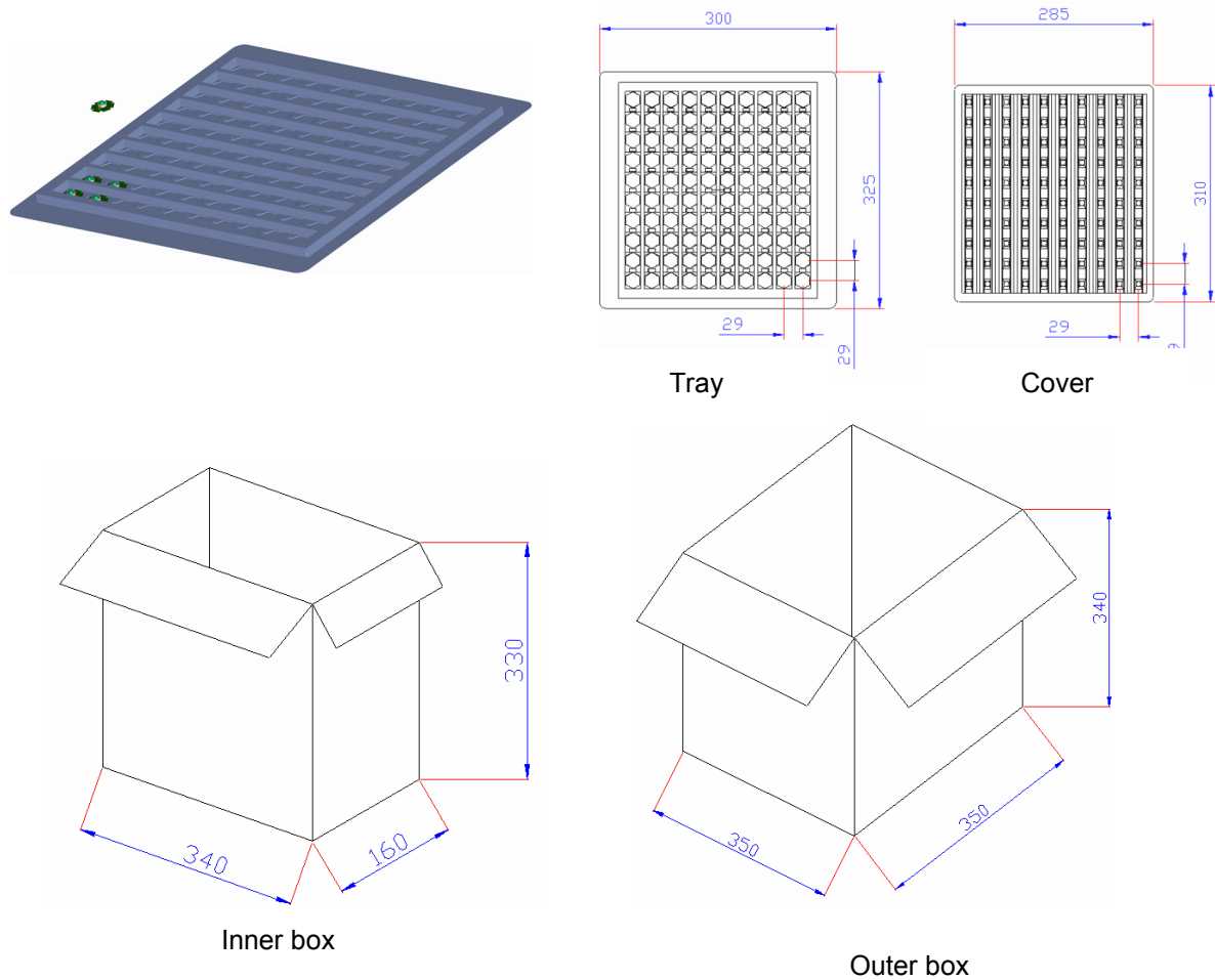
<Figure 33 Edixeon® star package and dimensions >
