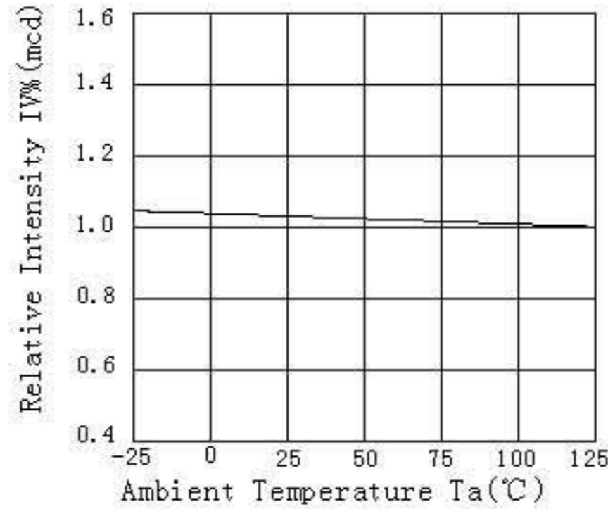
Relative Intensity vs. Ambient Temperature
