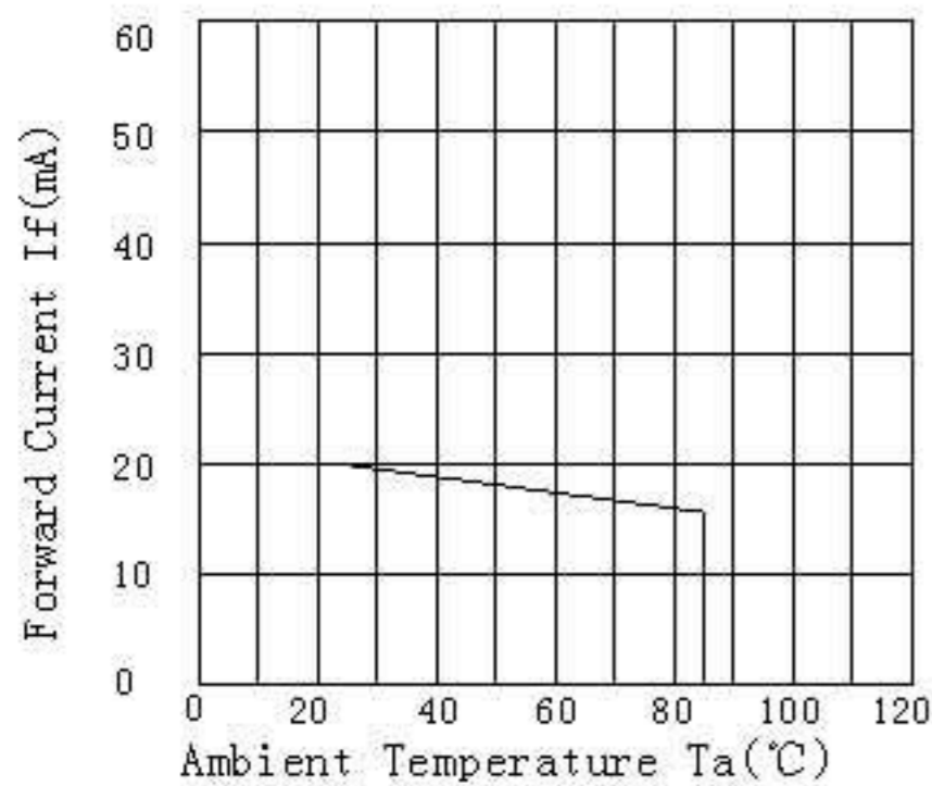
Forward Current vs. Ambient Temperature
