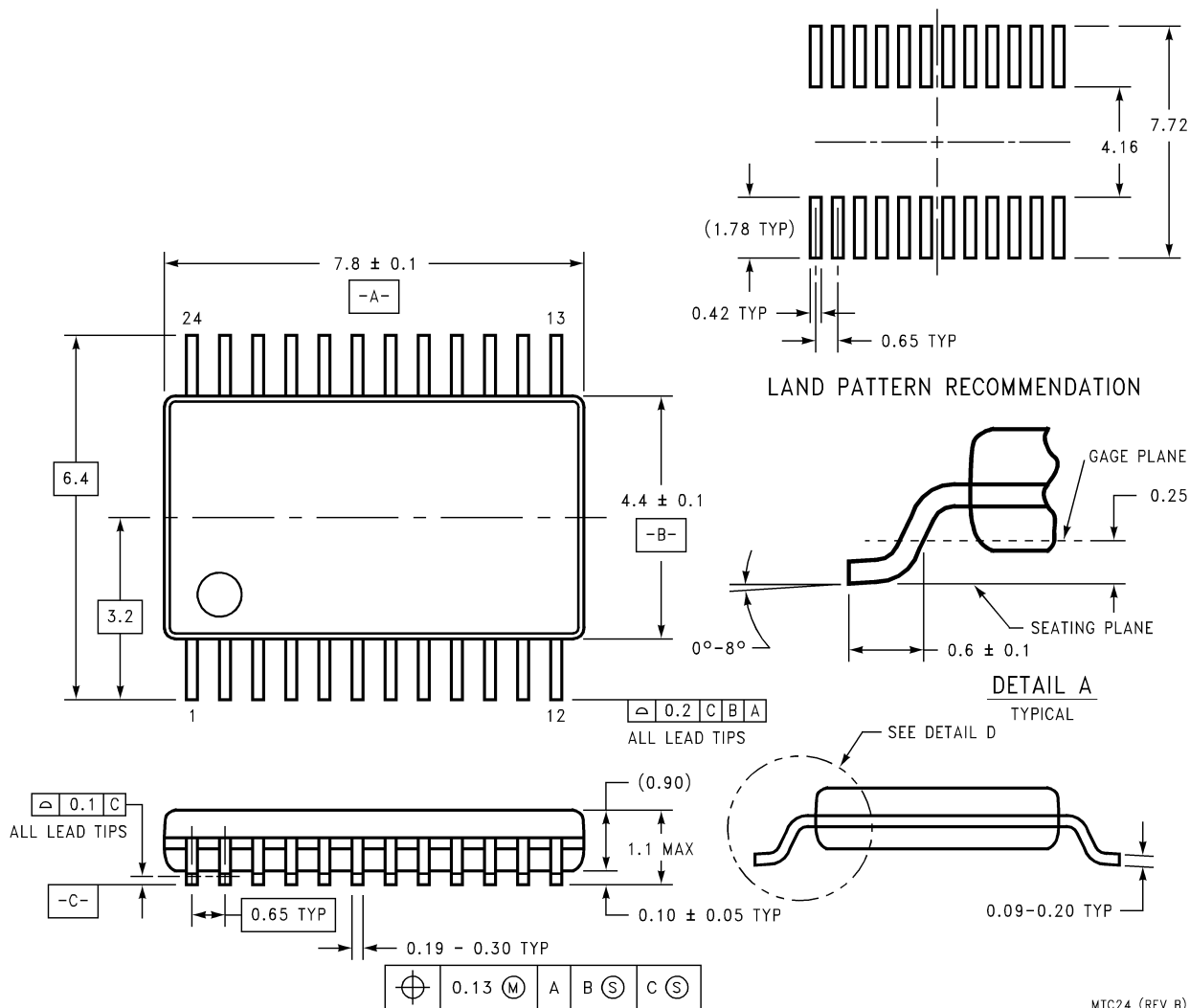
24-Lead TSSOP Order Number LM87C1MT NS Package Number MTC24B
